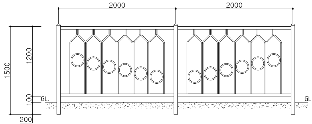
ELEVATION SCALE : NONE
