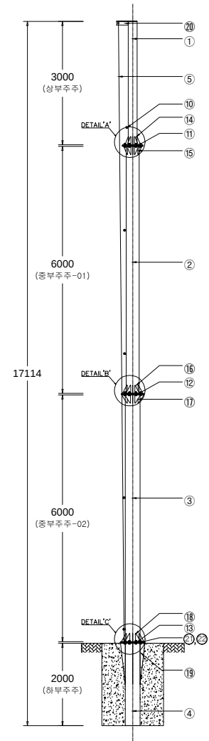
SIDE ELEVATION SCALE : NONE
