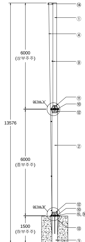
SIDE ELEVATION SCALE : NONE
