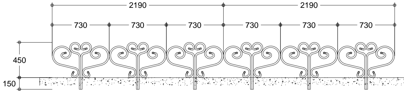
ELEVATION SCALE : NONE
