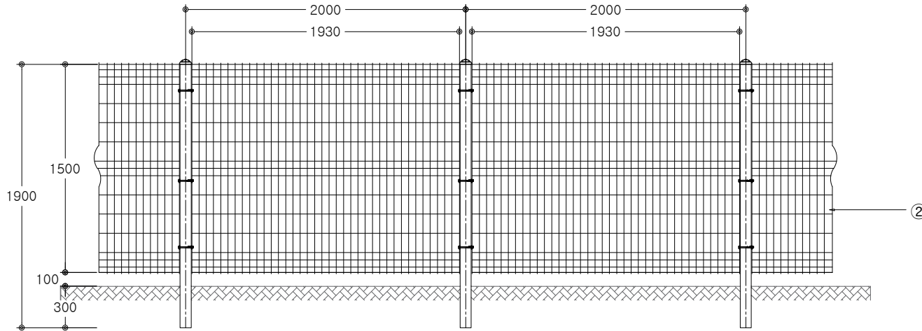
ELEVATION SCALE : NONE
