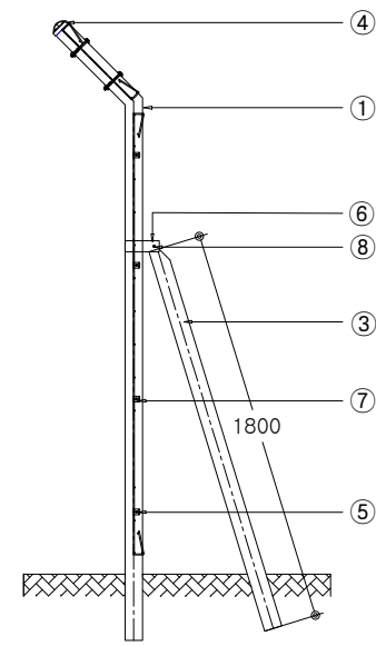
SIDE ELEVATION SCALE : NONE
