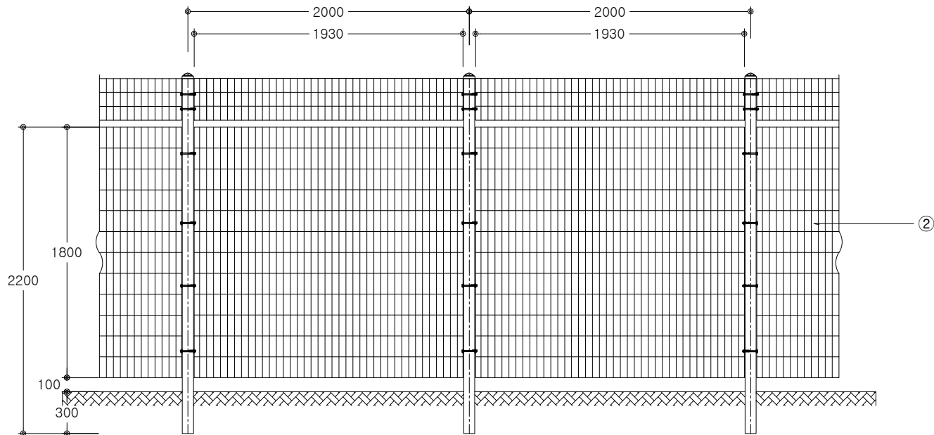
ELEVATION SCALE : NONE
