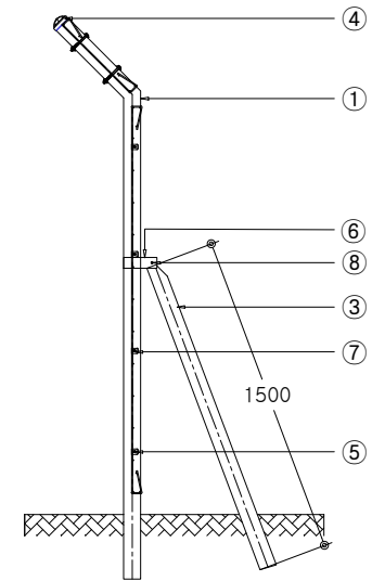
SIDE ELEVATION SCALE : NONE
