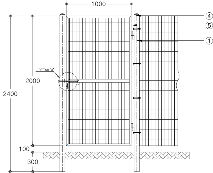
ELEVATION SCALE : NONE
