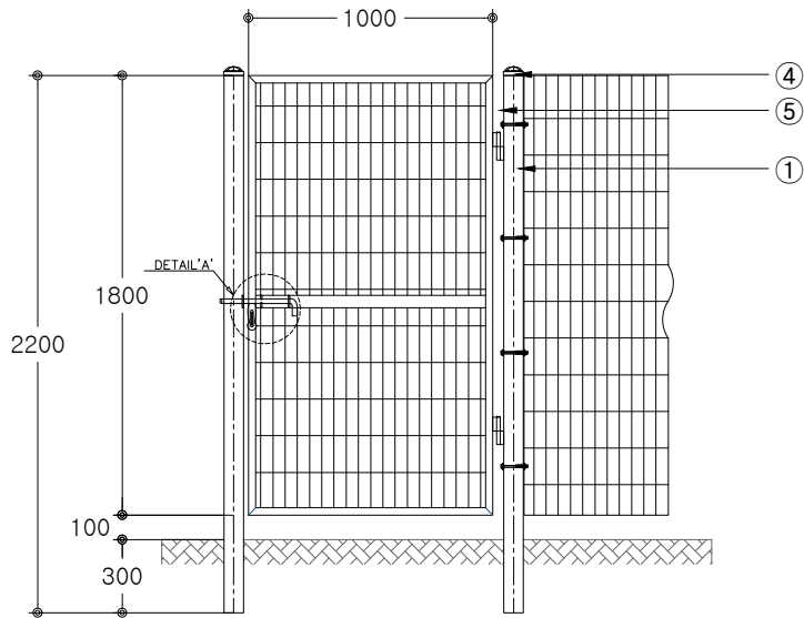
ELEVATION SCALE : NONE
