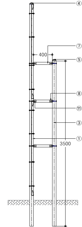
SIDE ELEVATION SCALE : NONE
