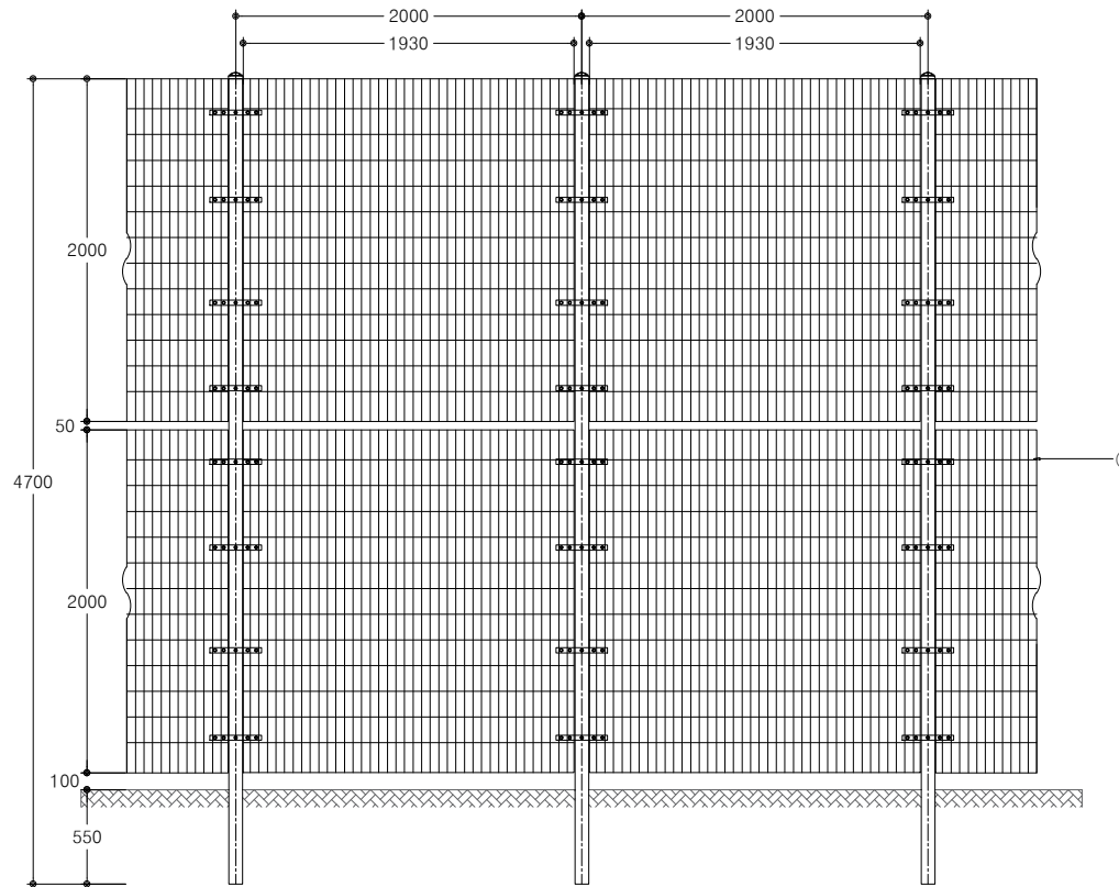
ELEVATION SCALE : NONE
