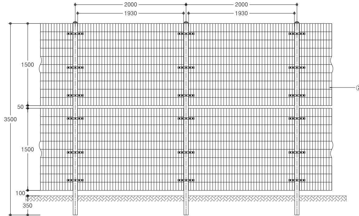
ELEVATION SCALE : NONE
