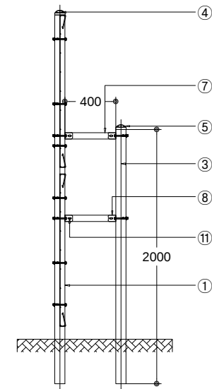
SIDE ELEVATION SCALE : NONE
