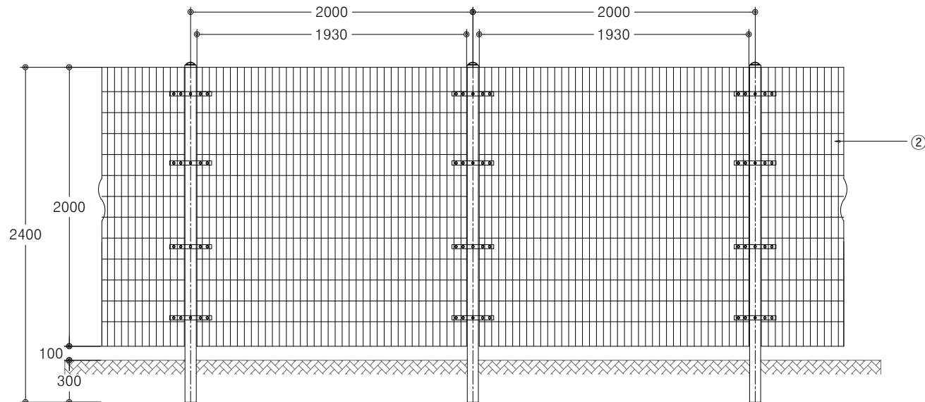
ELEVATION SCALE : NONE
