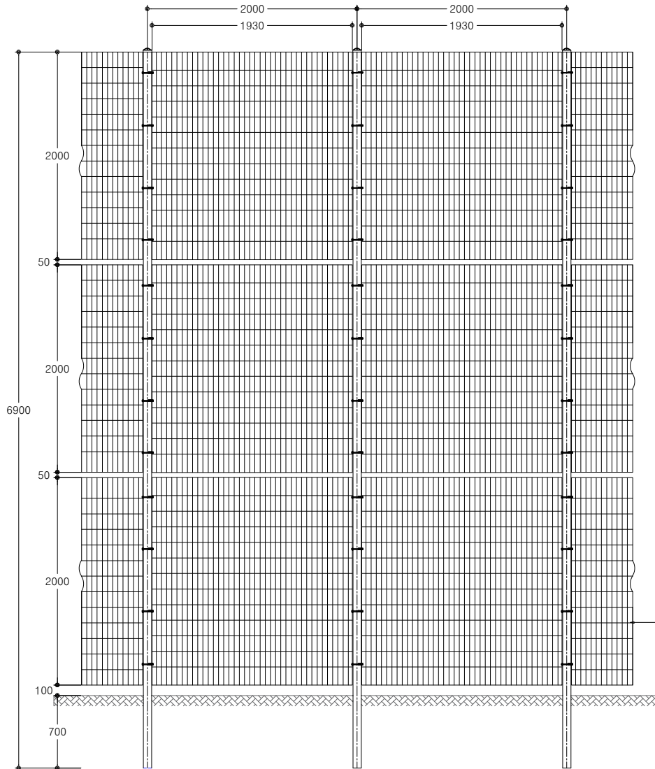
ELEVATION SCALE : NONE
