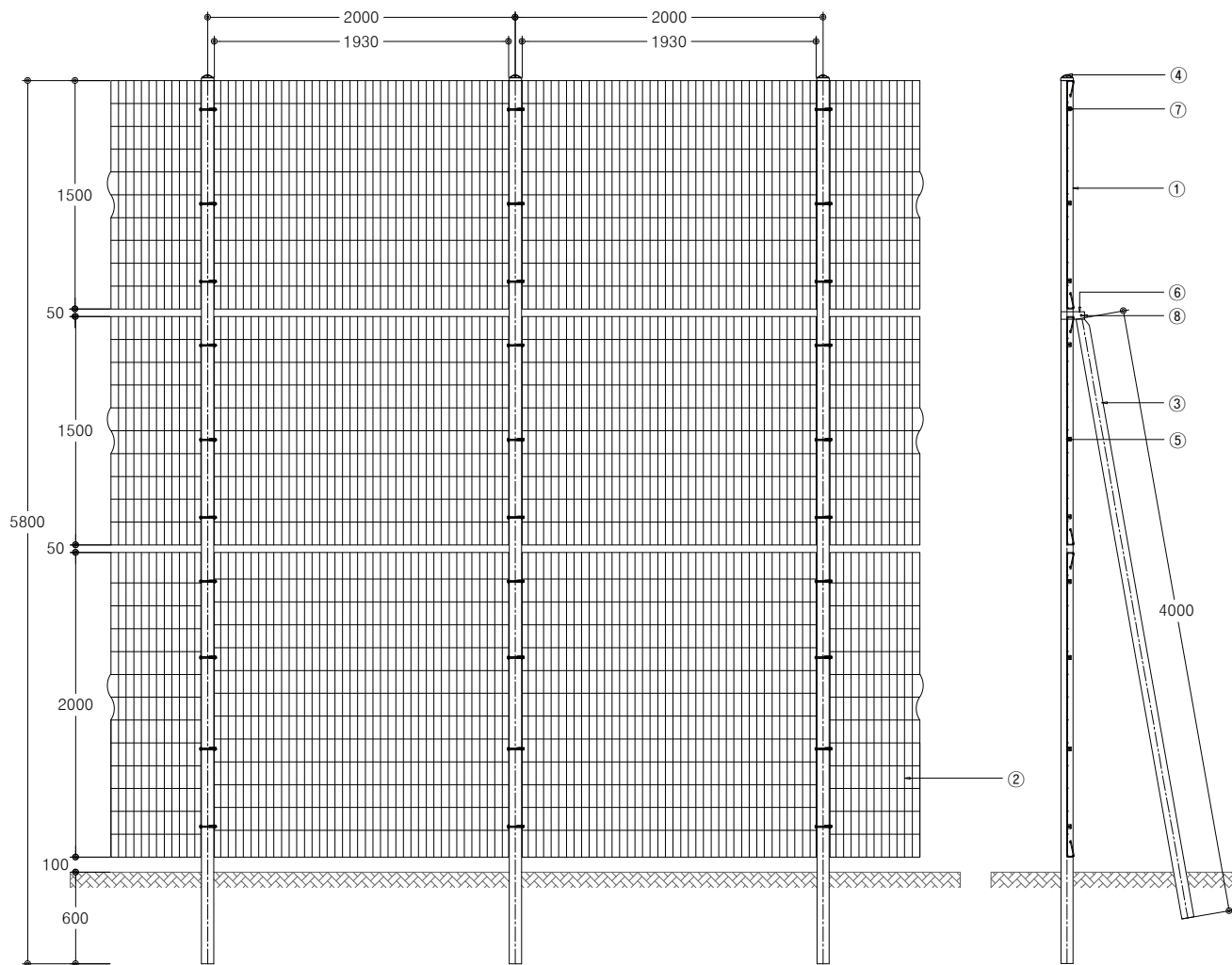
ELEVATION SCALE : NONE
