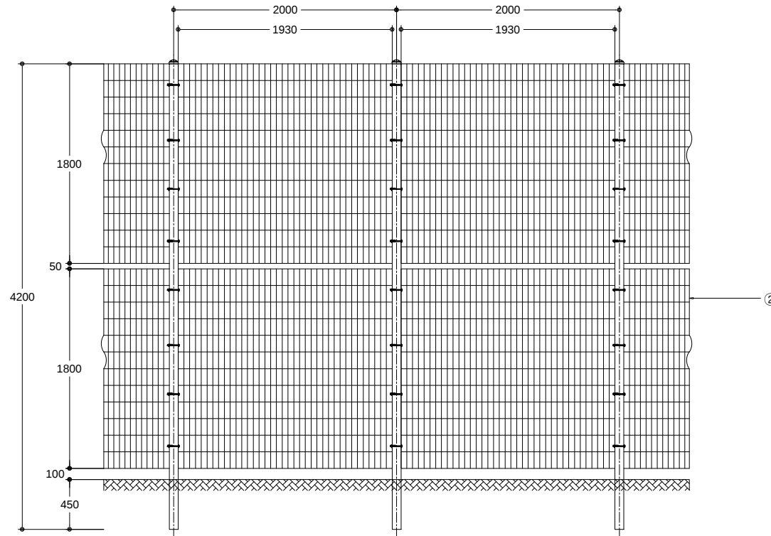
ELEVATION SCALE : NONE
