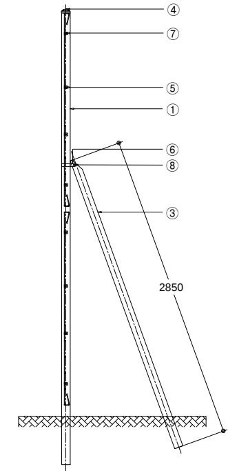
SIDE ELEVATION SCALE : NONE
