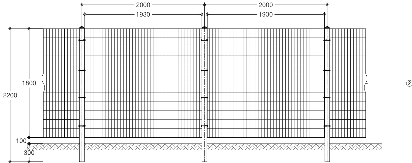
⊙ ELEVATION SCALE : NONE
