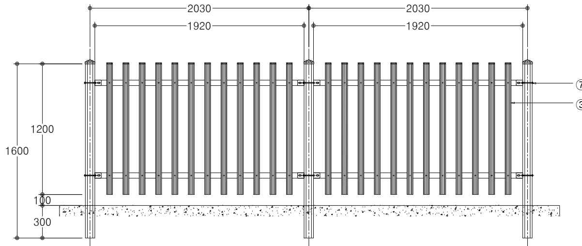
ELEVATION SCALE : NONE
